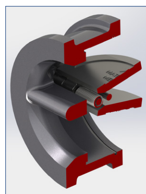
The Abacus Twin Plate check valve (rotated 90°).
