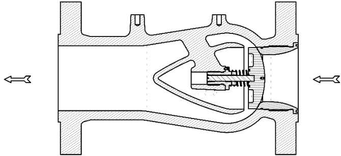
Fig.2 Valve Closed
